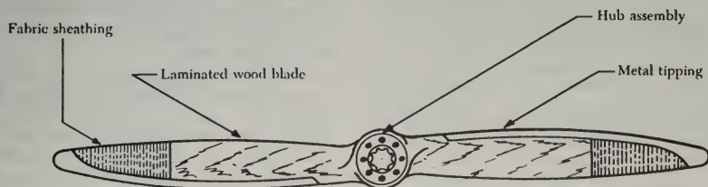
FIGURE 7-7. Fixed-pitch wooden propeller assembly.
